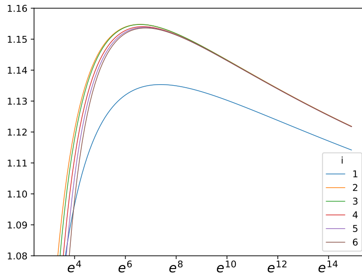
Figure 3: Plot of the functions u \mapsto \mathbf{Q}^{(i)}(\mathcal{X}(u), \mathcal{Y}(u)) for 1 \leq i \leq 6 , see Corollary 1.
