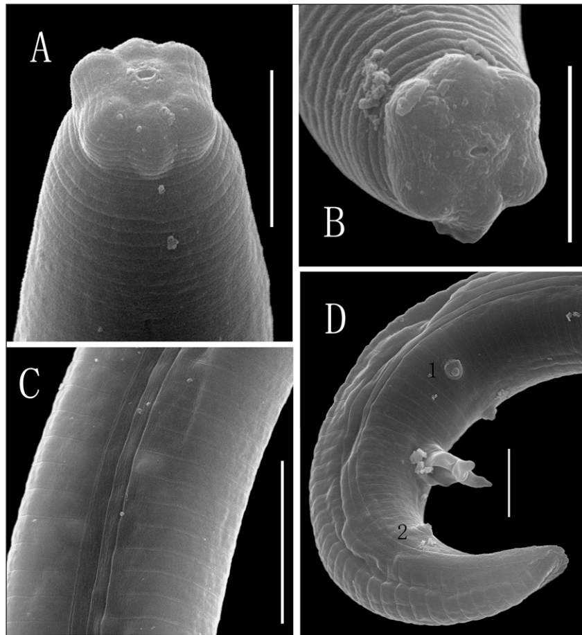
Scanning electron micrographs (SEM) of Ektaphelenchus macrobulbosus
