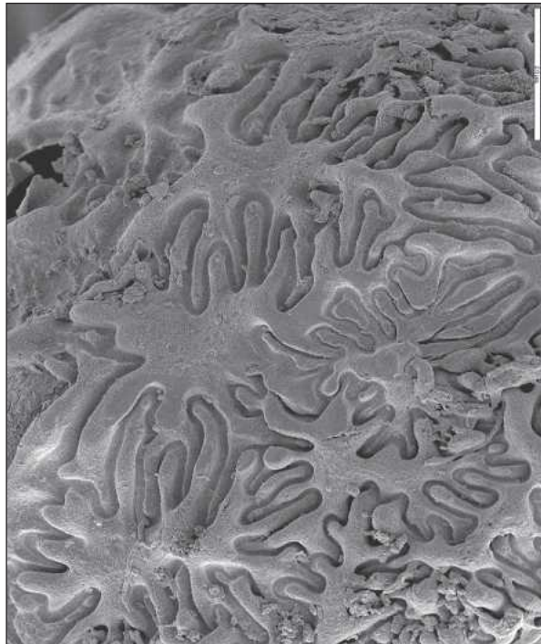
Spines and surface markings of the Meloidoderita kirjanovae cystoid body
