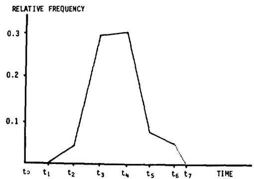
FIG. 1. Relative frequency of Meloidogyne larvae in roots (curve shown is for female second-stage M. incognita larvae developing at 20 C).
