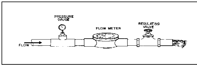
Figure 2. Pump capacity measuring apparatus, including a pressure gauge, flow meter, and regulating valve.
