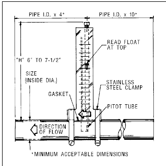
Figure 1. Pitot tube flow rate meter.
