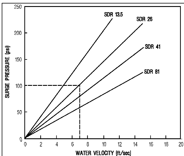
Figure 1. Surge pressure levels associated with a valve closure for different levels of pipeline water velocity. (For 400,000 psi modulus of elasticity PVC material)
