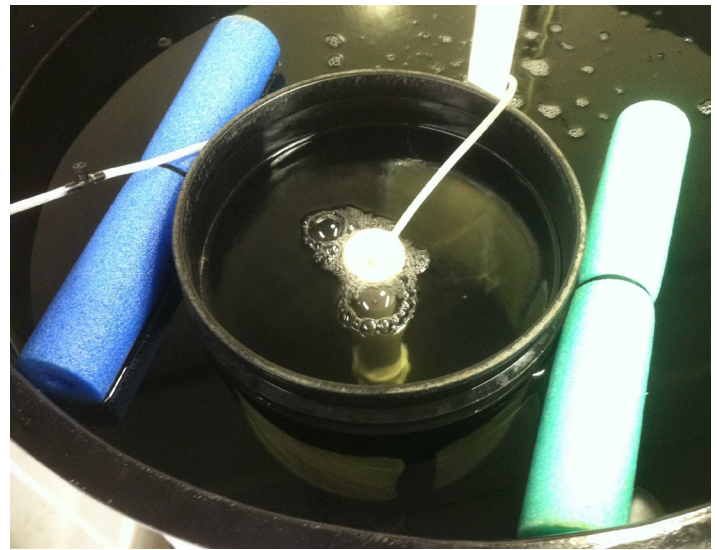
Figure 3. An airlift collector functioning properly in a copepod culture tank. Credit: Jason S. Broach
