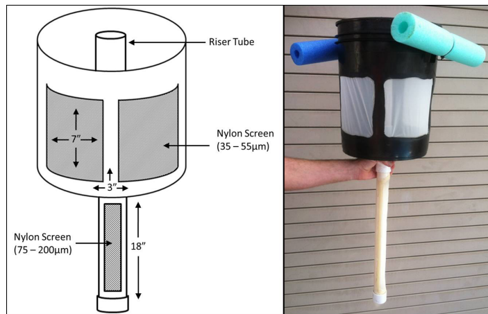
Figure 1. Floating airlift used in the collection of live-feed organisms. Credit: Jason S. Broach
