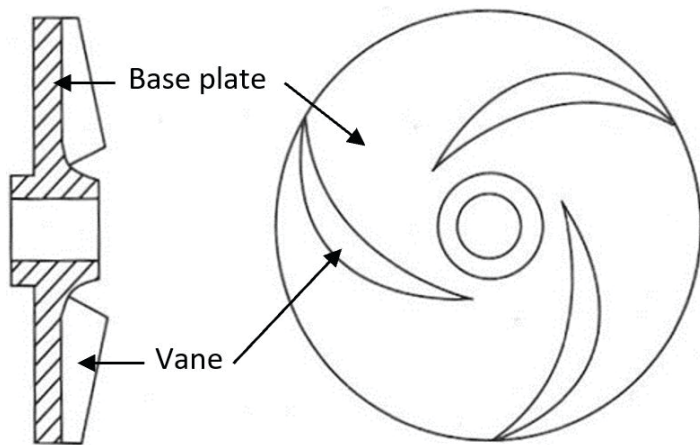
Figure 4. Semi-closed impeller. Credits: Wheaton (1977)
