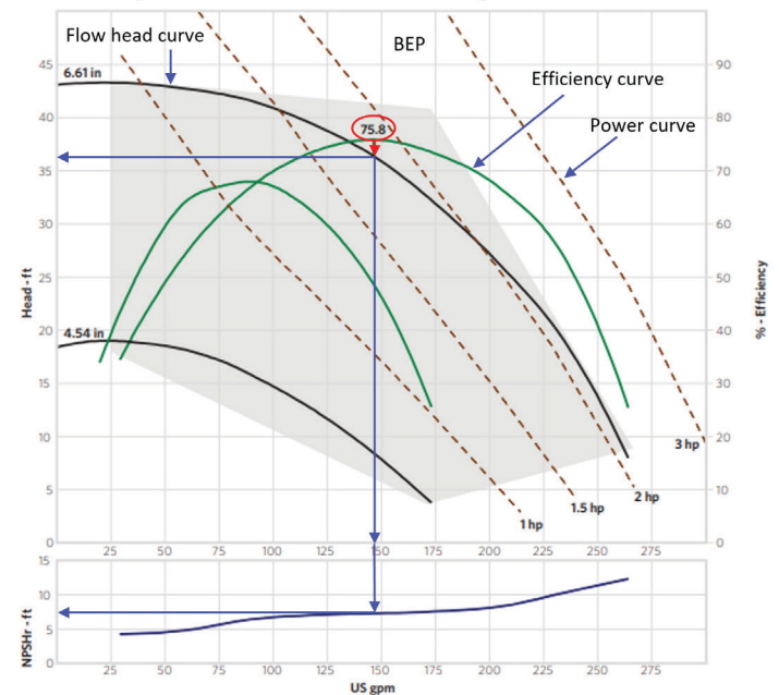
Figure 7. Pump performance diagram for a pump with an impeller diameter between 4.54 and 6.61 inches.
