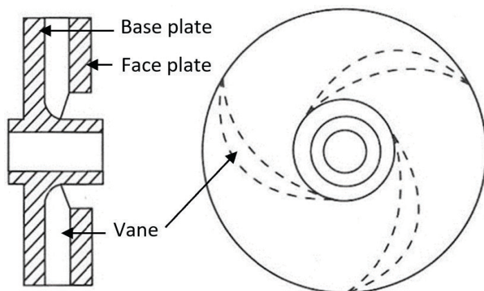
Figure 5. Closed impeller. Credits: Wheaton (1977)
