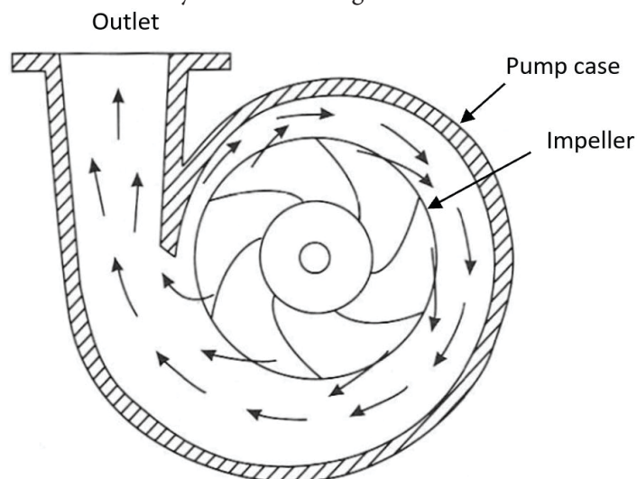
Figure 1. Volute centrifugal pump. Credits: Wheaton (1977)
