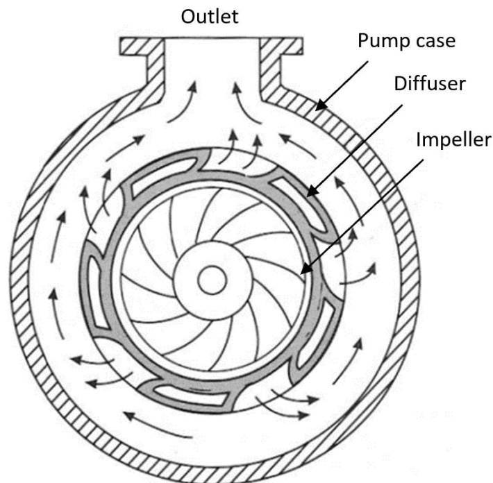
Figure 2. Diffuser centrifugal pump. Credits: Wheaton (1977)
