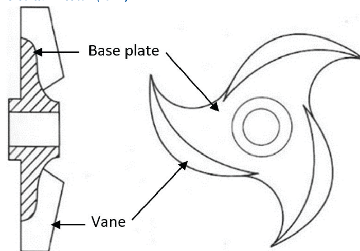
Figure 3. Open impeller. Credits: Wheaton (1977)
