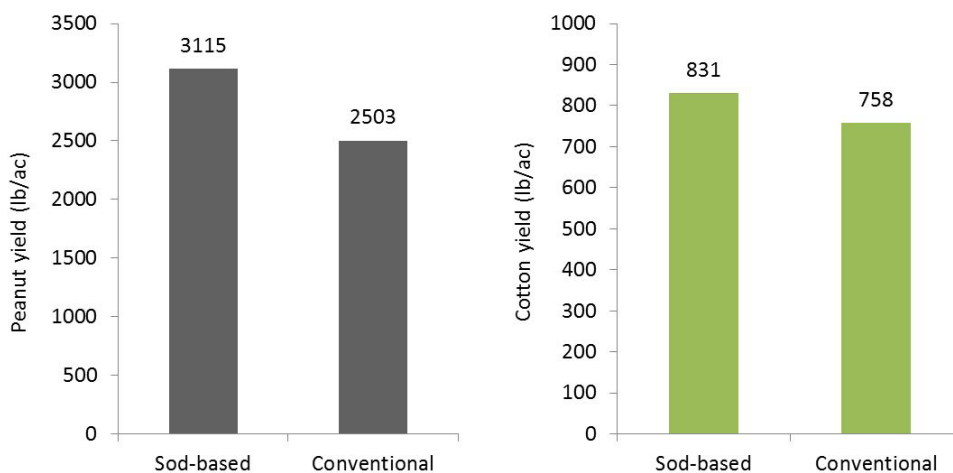
Figure 2. Yield differences in peanut and cotton for sod-based and conventional rotations, using averages of dryland and irrigated fields for 2002-2004 (data from Katsvairo et al. 2007).
