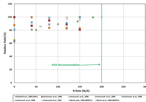
Figure 2. Response of potato to N fertilization with sprinkler irrigation in Florida.
