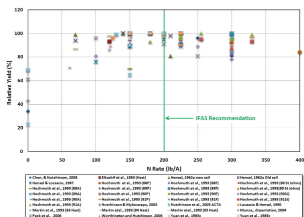
Figure 3. Potato yield responses to rates of N fertilizer with subsurface irrigation.
