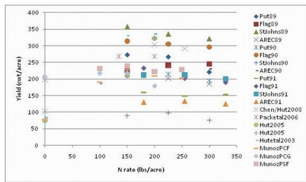
Figure 9. Potato yield versus N rate for more recent studies that included at least 3 levels of N, with other nutrients held constant. These values are the same data as in Figure 7, but here the actual yield in cwt/acre instead of the percent relative yield are presented. The first 11 studies were Hochmuth et al., 1993b; Other reports are Chen and Hutchinson, 2008; Pack et al., 2006; Hutchinson, 2005; Hutchinson et al., 2003; and Munoz, 2004.
