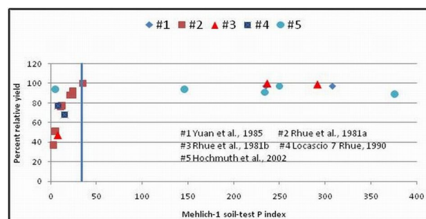
Figure 11. Response of potato yield on soils with variable residual Mehlich-1 P concentrations (without P fertilization). Vertical blue line denotes current M-1 cut-off (30 ppm) between medium and high soil test indexes.
