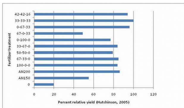
Figure 6. Potato yield response to three N CRF products (A, B, C; 33% release) engineered to release completely by 120, 75, and 45 days after application mixed in various percentages (x-x-x) for fertilization of potato (Hutchinson, 2005).
