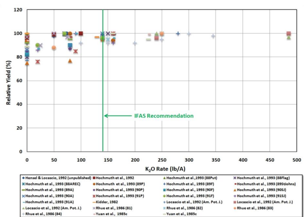
Figure 13. Relative yield of potatoes for experiments, years, seasons, and irrigation systems as a function of added K 2 O.
