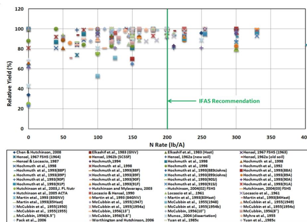
Figure 4. Response of potato to N fertilization with all irrigation methods in Florida.
