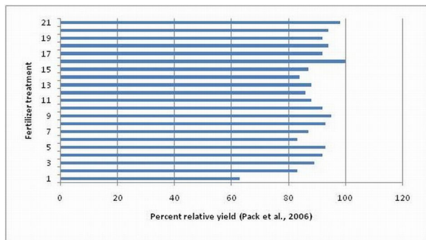
Figure 5. Potato response to several controlled-release nitrogen fertilizers (Pack et al., 2006). Treatment 1 was the control (0 N); treatments 2 through 4 were soluble N at 0, 130, or 220 lb/acre; the remaining treatments were various CRF programs.
