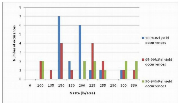
Figure 8. Plot of number of occurrences for three yield levels versus the N rate from studies summarized in Fig. 7. We chose to group the responses (90 to 94%) and 95 to 99% for easier viewing. There were no instances where 95% to 99% percent relative yields were significantly different from 100% relative yield. The reader will note that numbers of observations for each N rate varied.
