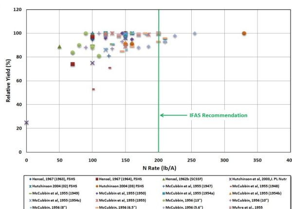
Figure 1. Relative yield of potatoes for experiments, years, and seasons (in parens) as a function of added N (mixed fertilizer).
