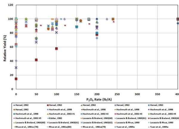
Figure 12. Relative yield of potatoes for experiments, years, seasons, and irrigation systems as a function of added P_2O_5 .
