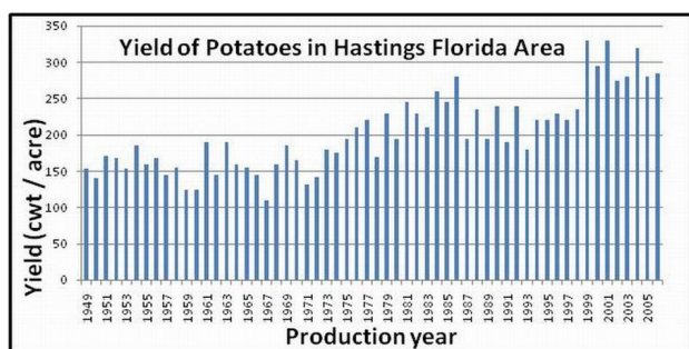
Figure 10. Yield of potato over years for Hastings, Florida production area. Yield has generally increased (nearly doubled) since 1949, but there are variations in yield from year to year. Data are from http://usda.mannlib.cornell.edu/usda/ers/91011/Table010.xls .
