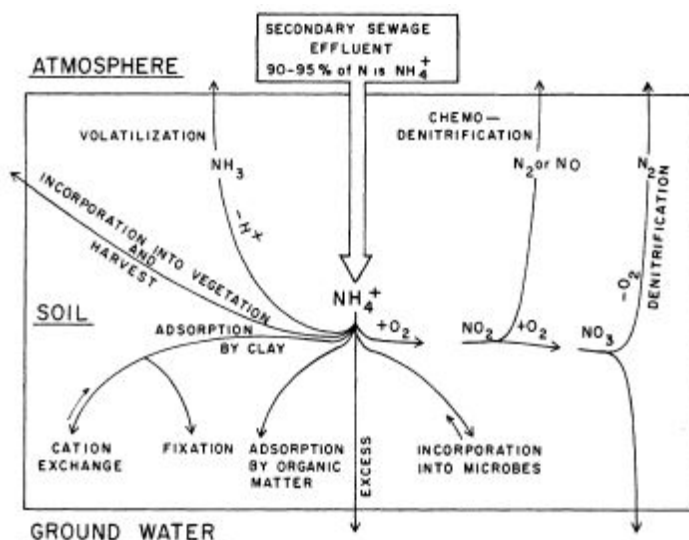
Figure 2. Nitrogen transformations below a septic system drain field. (Source: Lance 1972).
