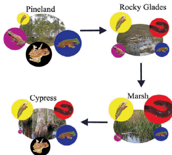
Figure 6. Diagram showing how the proportion of an area occupied (PAO) by various amphibian species might differ in four habitat types. Arrows indicate direction of increasing hydroperiod from very few days in pineland habitat to almost permanent inundation in cypress habitat. The size of the circle around each amphibian species indicates the PAO for that species in that habitat. Little Grass Frogs (pink circle) are relatively abundant in pine-lands, but decrease in terms of PAO in the wetter habitats. Greater Sirens (red circle) are only found in wetter habitats, but reach their largest PAO in open marsh habitats. Credits: Hardin Waddle, 2004
