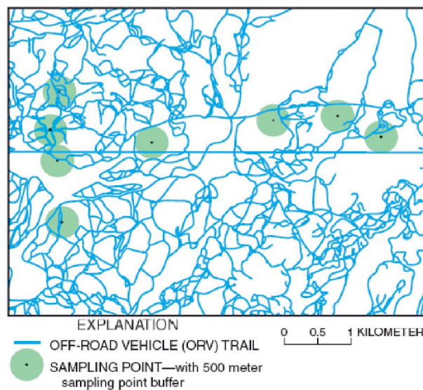
Figure 7. Eight sampling points with a surrounding 500-meter buffer. The blue lines are off-road vehicle (ORV) trails, and the length of ORV trail segments within the green circles is the basis of the ORV index. Credits: Hardin Waddle 2004; Adapted from Welch, et. al 1998
