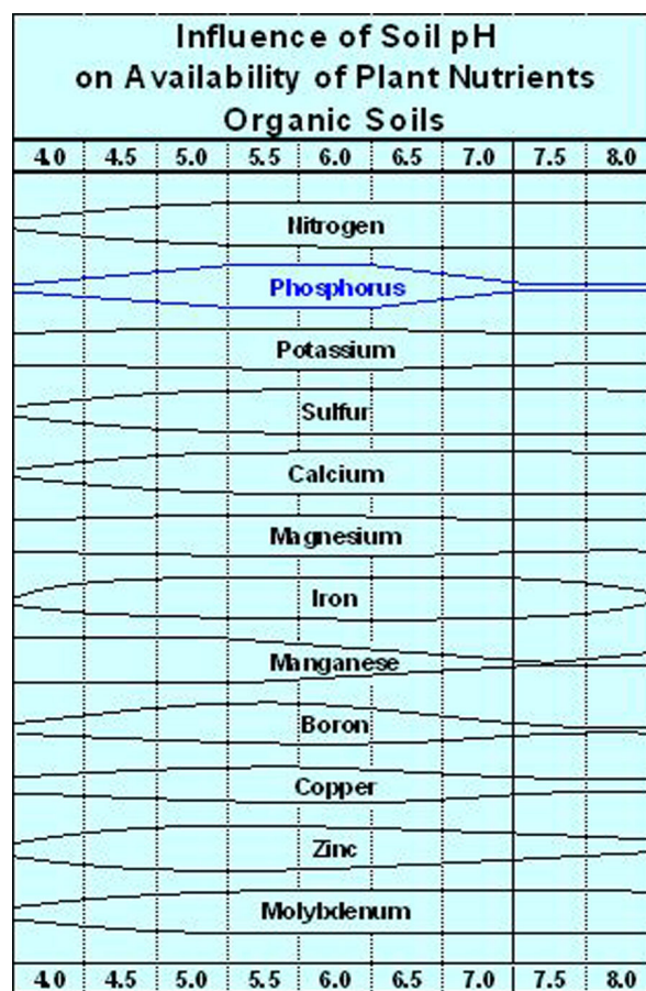
Figure 2. Influence of soil pH on nutrient availability in organic soils (Lucas, 1982).
