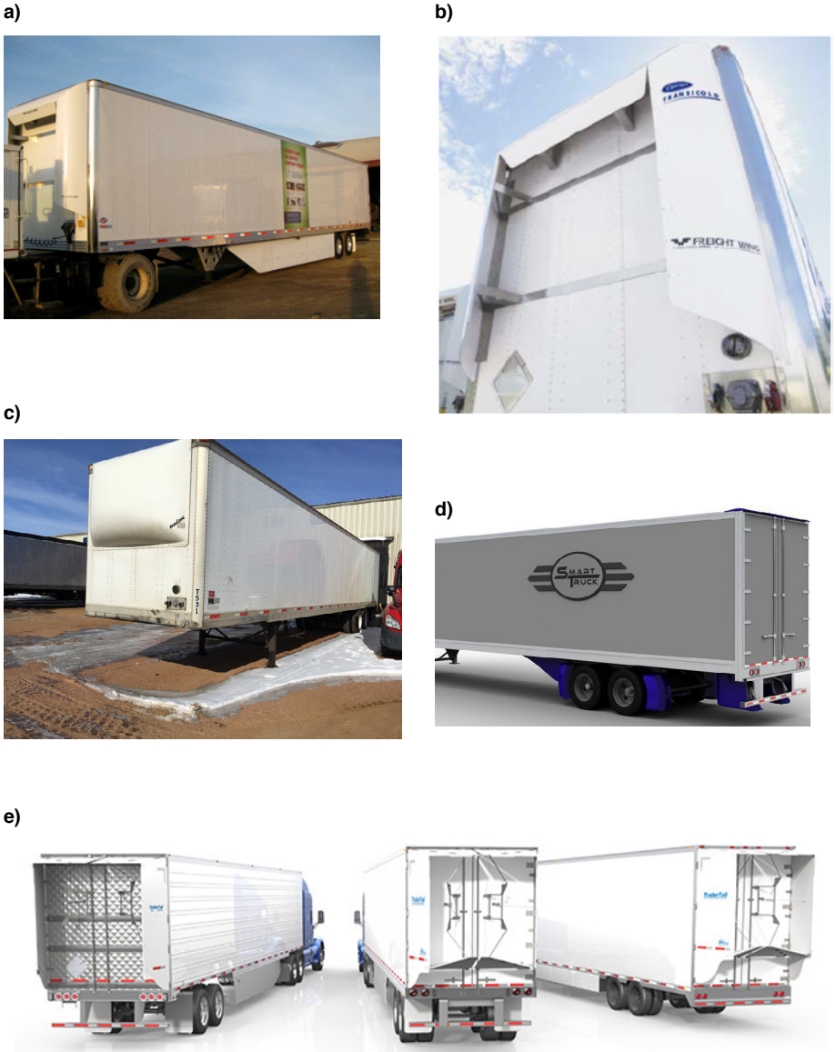
Figure 16. Airfoil accessories to increase fuel efficiency. a) nose cone, b) gap fairing between tractor and trailer, c) belly fairing, d) underbody fairings, e) boat tails. (Source: Curry et al., 2012; https://www.theicct.org/publications/reducing-aerodynamic-drag-and-rolling-resistance-heavy-duty-trucks )
