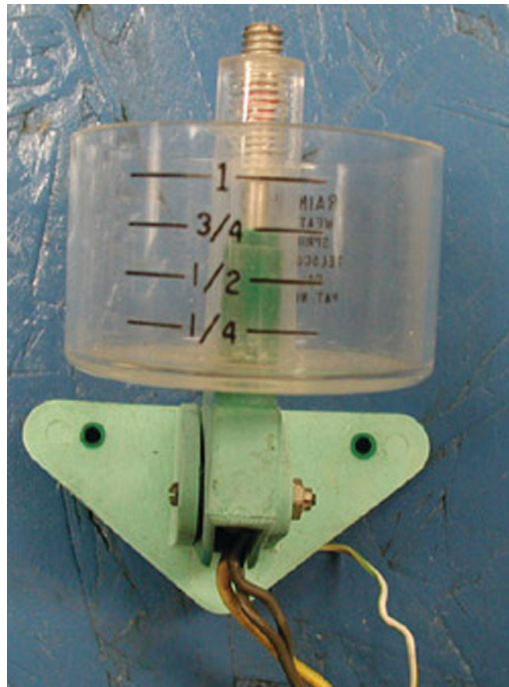
Figure 1. Weight-based rain shutoff device.
